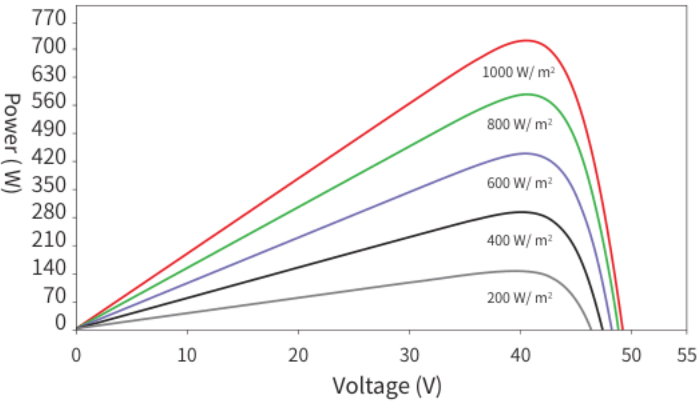
Power-Voltage Curves (66HL5-BDV 725W)
