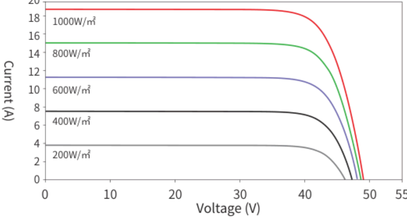
Current-Voltage Curves (66HL5-BDV 725W)
